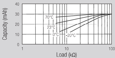
Cell capacity at various loads
