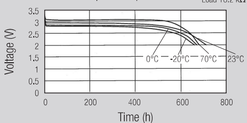
Temperature performance
