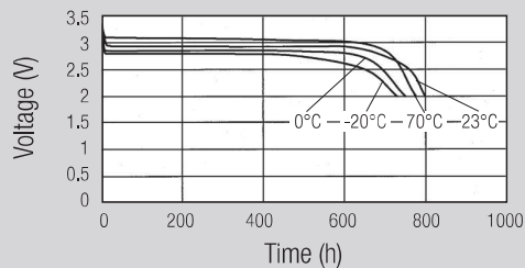
Temperature performance Load 12 kΩ
