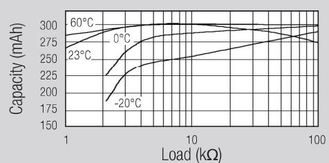
Cell capacity at various loads
