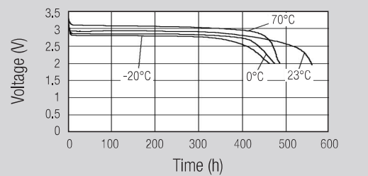
Temperature performance
