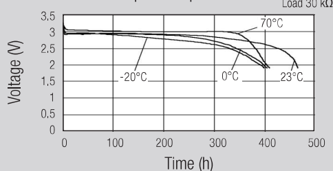
Temperature performance
