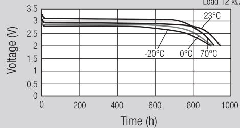
Temperature performance
