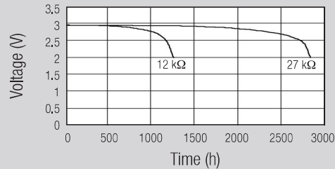
Discharge performance at 23°C
